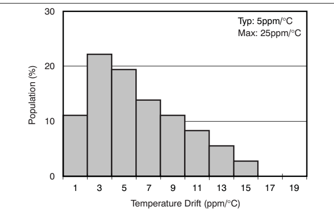
Figure 5. Reference Output Temperature Drift (-40°C to +125°C, Grades A and B)
