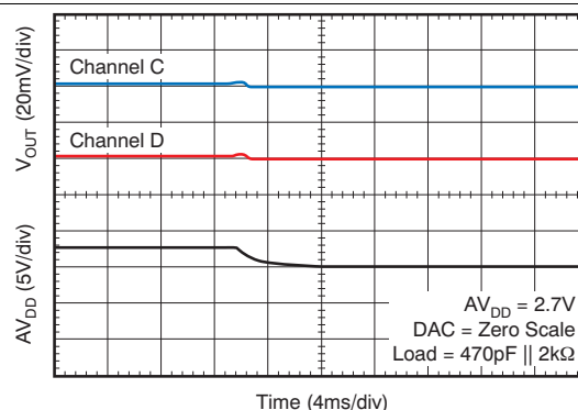
Figure 113. Power-Off Glitch
