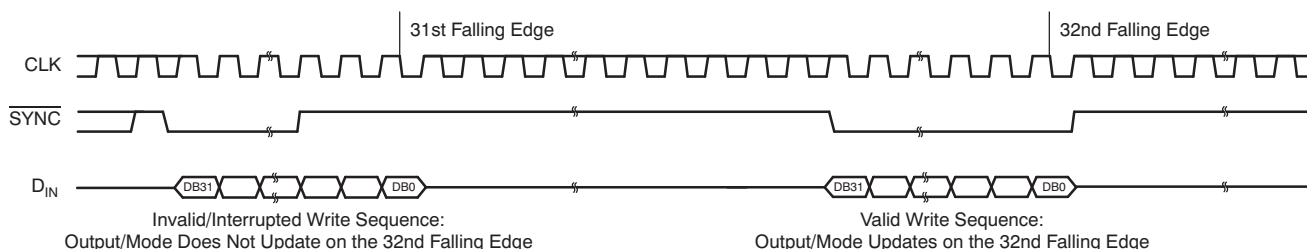
Figure 123. \overline{\text{SYNC}} Interrupt Facility
