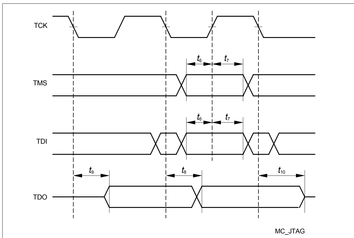
Figure 27 JTAG Timing
