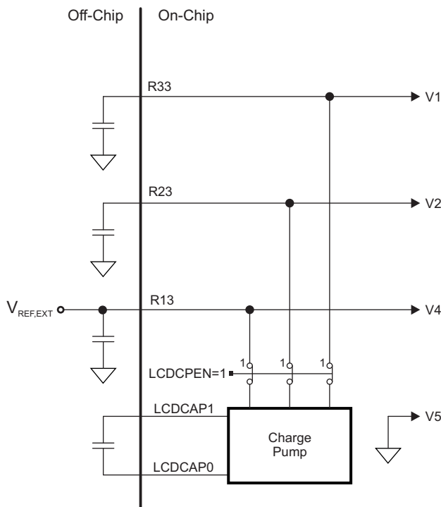
Figure 17-11. LCD Operation Mode 4
