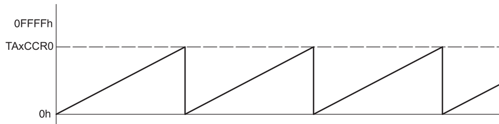
Figure 13-2. Up Mode
