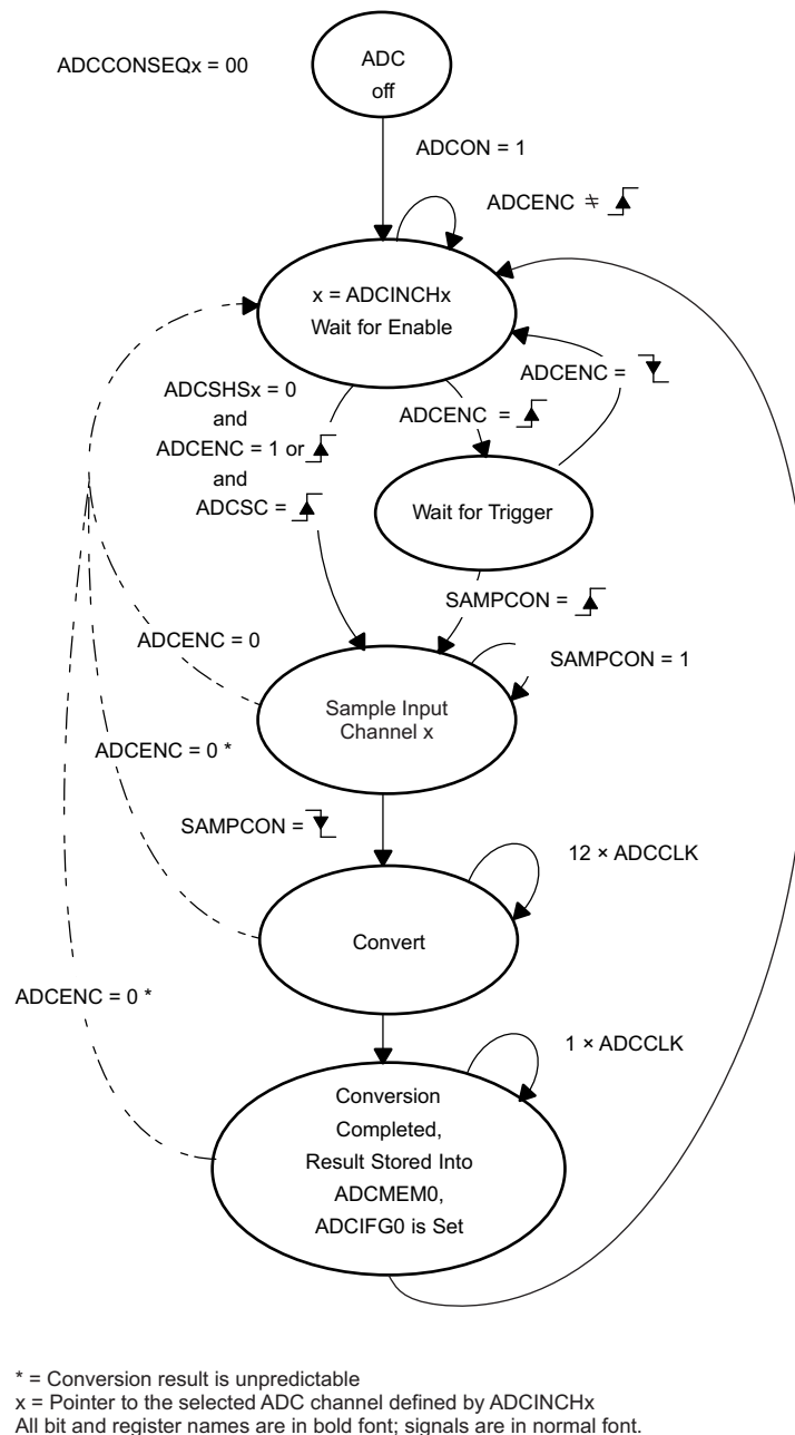
Figure 21-10. Single-Channel Single-Conversion Mode in 10-Bit Mode
