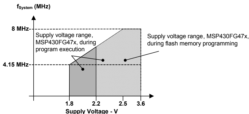
Figure 1. Frequency vs Supply Voltage, Typical Characteristics
