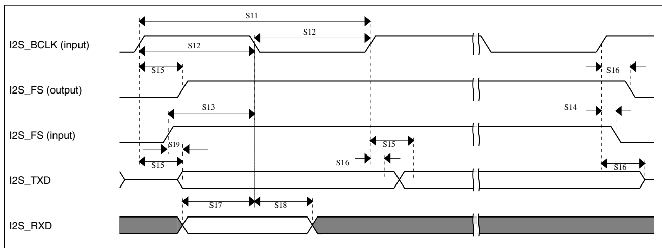
Figure 40. I 2 S timing — slave modes
