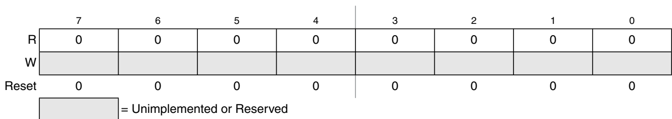
Figure 17-18. Flash Reserved2 Register (FRSV2)
