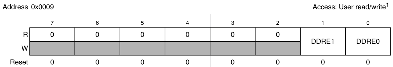
Figure 2-2. Port E Data Direction Register (DDRE)
