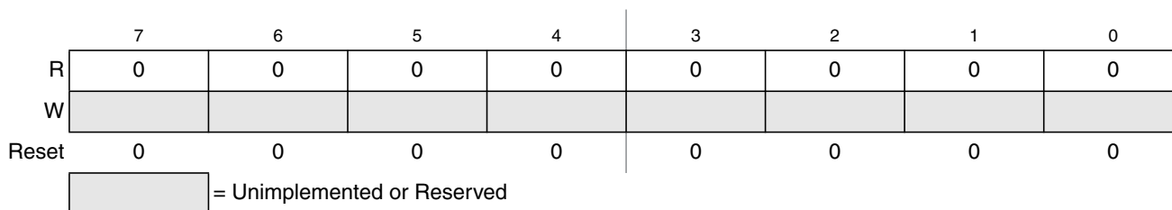
Figure 17-19. Flash Reserved3 Register (FRSV3)
