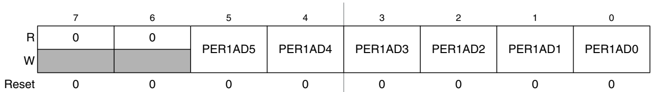
Figure 2-41. Port AD Pullup Enable Register (PER1AD)
