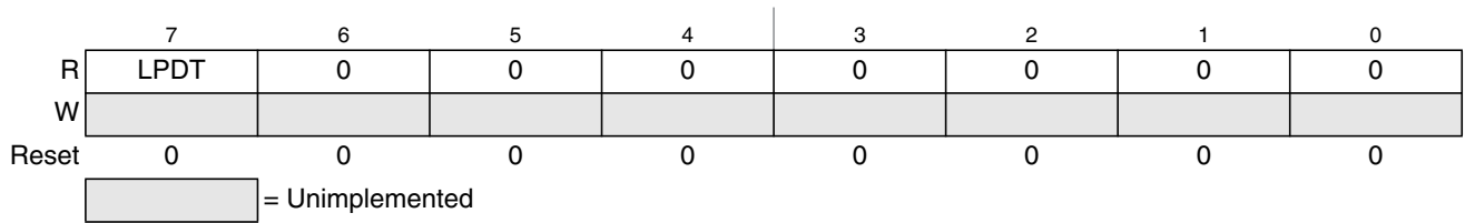
Figure 15-8. LIN Status Register (LPSR)
