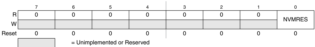
Figure 3-7. MMC Control Register (MMCCTL1)
