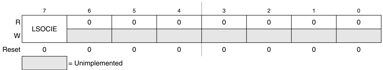
Figure 14-5. LSDRV Interrupt Enable Register (LSIE)
