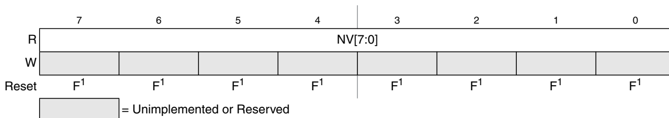
Figure 17-21. Flash Option Register (FOPT)
