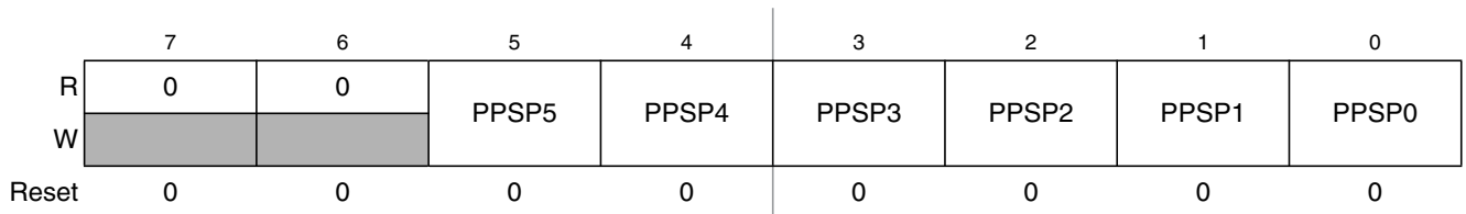
Figure 2-28. Port P Polarity Select Register (PPSP)
