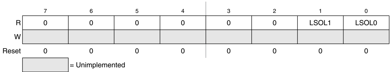
Figure 14-4. LSDRV Status Register (LSSR)
