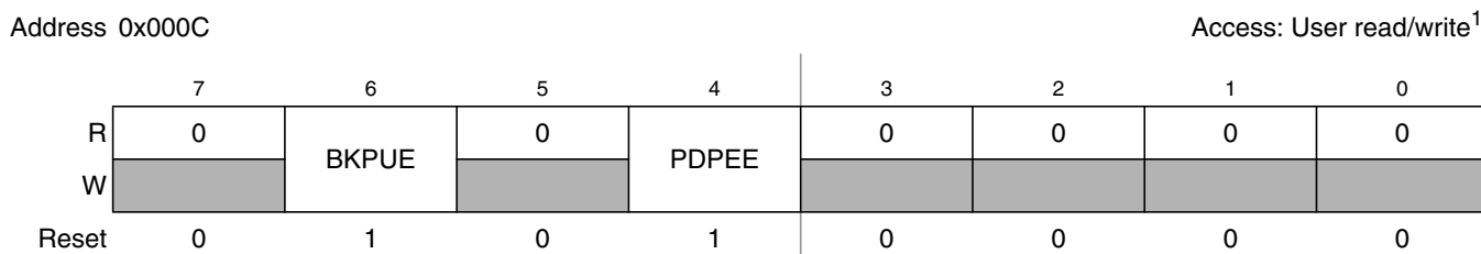
Figure 2-3. Port E, BKGD pin Pull Control Register (PUCR)
