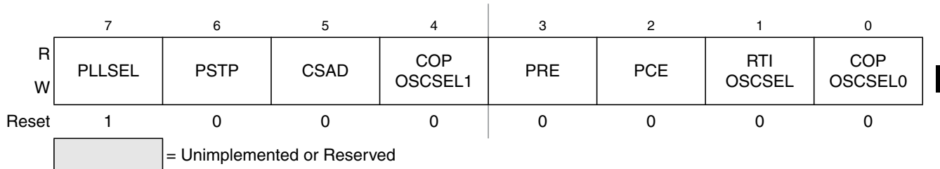
Figure 4-9. S12CPMU_UHV Clock Select Register (CPMUCLKS)
