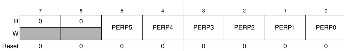
Figure 2-27. Port P Pull Device Enable Register (PERP)
