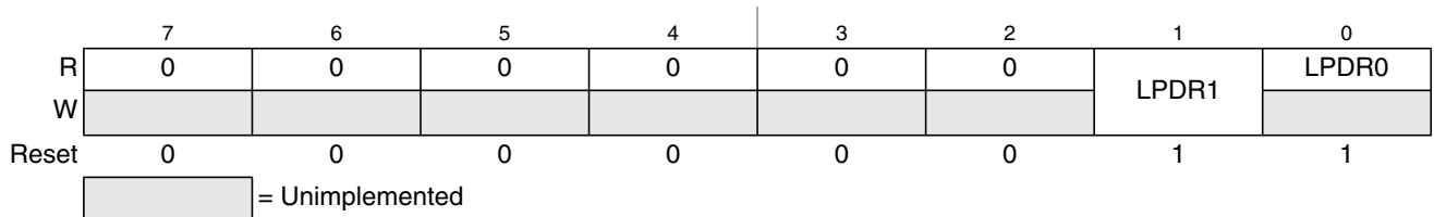
Figure 15-3. Port LP Data Register (LPDR)
