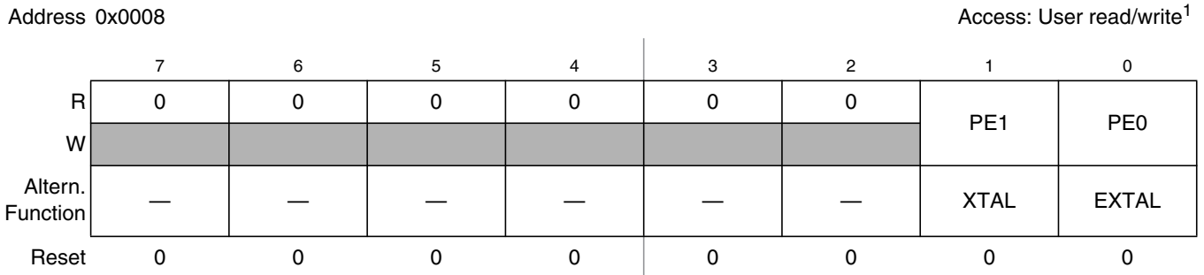
Figure 2-1. Port E Data Register (PORTE)
