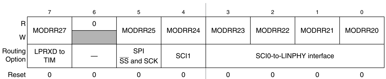
Figure 2-21. Module Routing Register 2 (MODRR2)
