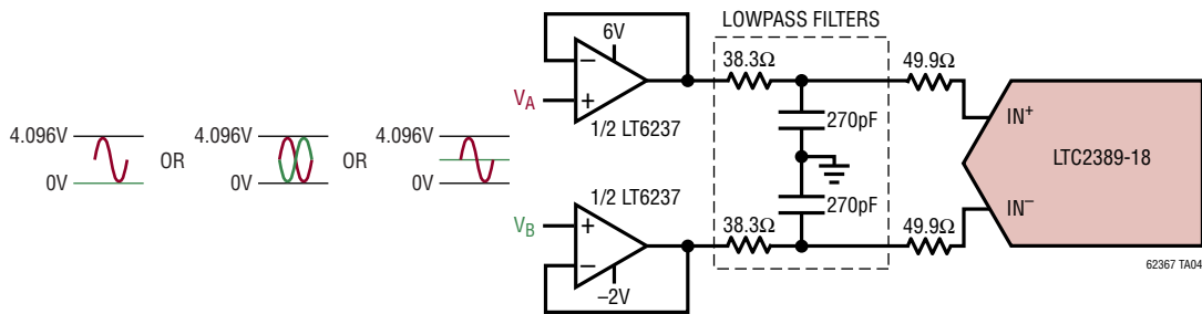
Driving a Fully Differential ADC
