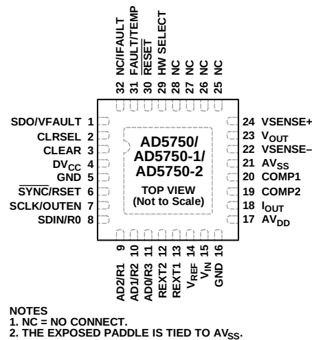
Figure 4. Pin Configuration
