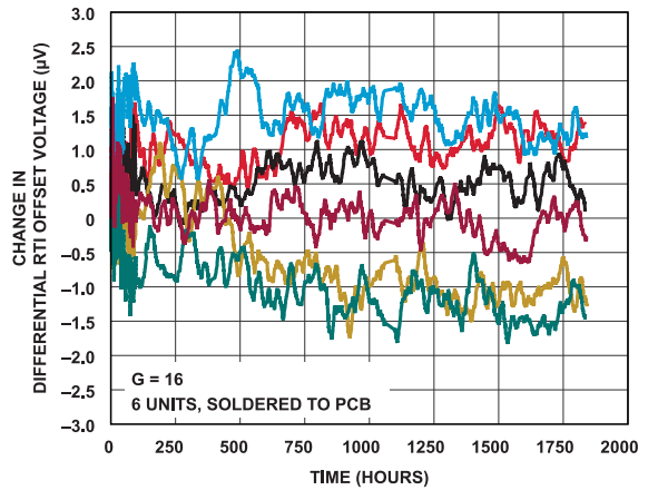
Figure 29. Long Term Differential RTI Offset Voltage Drift
