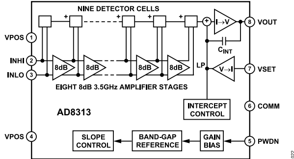
Figure 22. Block Diagram
