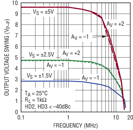
Maxium Undistorted Output Signal vs Frequency
