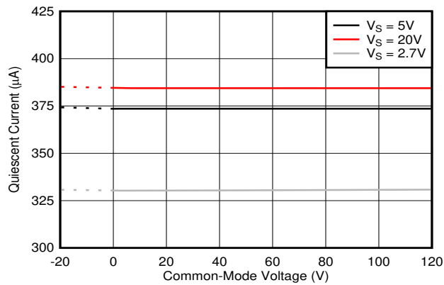
Figure 6-37. Quiescent Current vs. Common-Mode Voltage, INA2290
