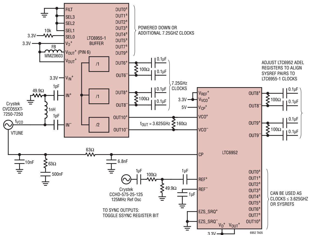
Generation of 7.25GHz, 52fs ADC SNR Jitter Clocks Using LTC6952 and LTC6955-1
