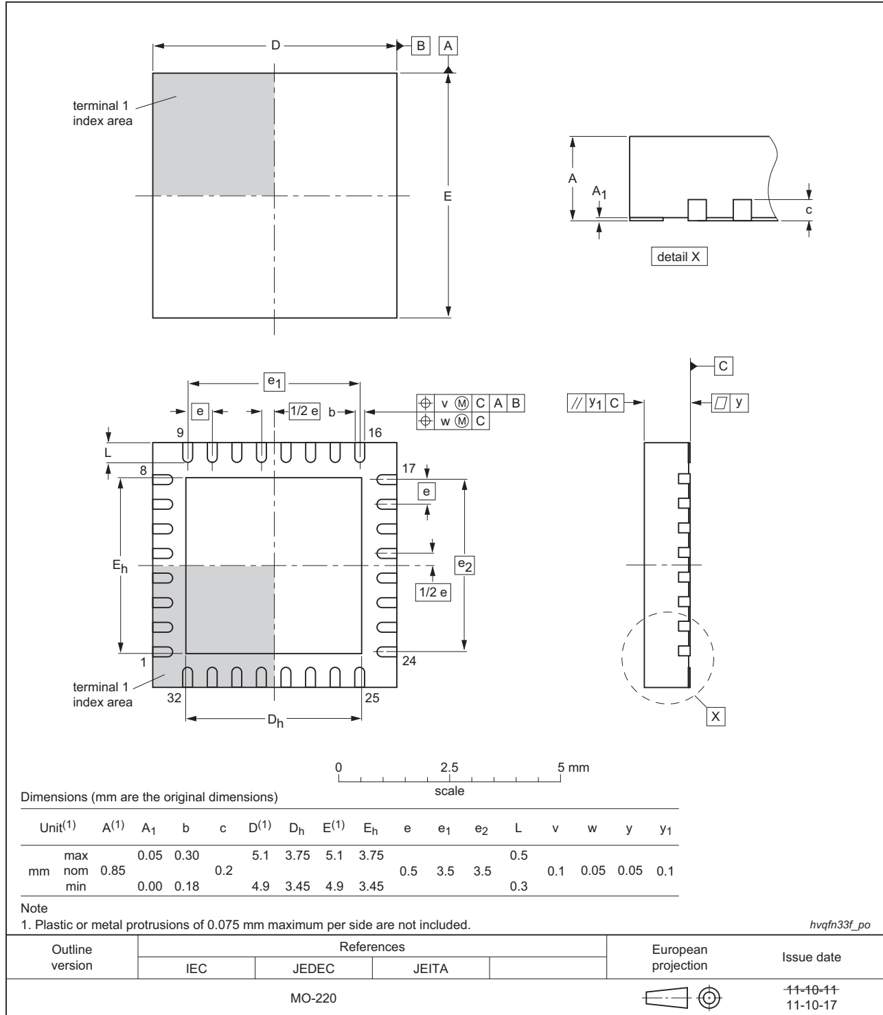
Fig 44. Package outline (HVQFN33 5x5)
