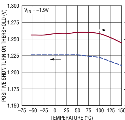
SHDN Turn-On Threshold
