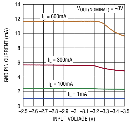
GND Pin Current Entering Dropout
