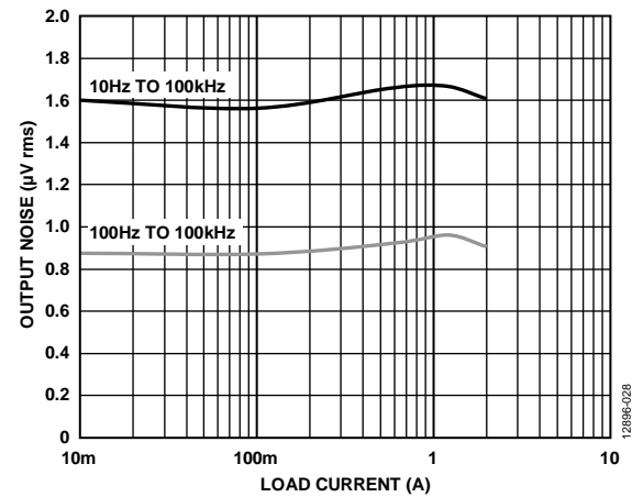
Figure 28. RMS Output Noise vs. Load Current
