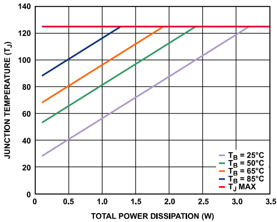
Figure 77. SOIC
