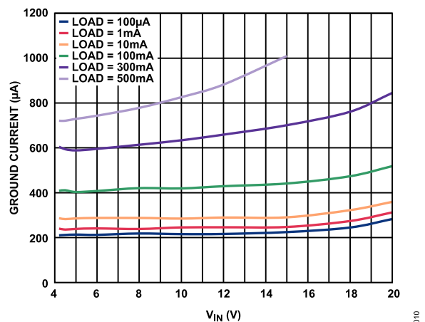
Figure 10. Ground Current ( I_{GND} ) vs. Input Voltage ( V_{IN} ), V_{OUT} = 3.3\text{ V}
