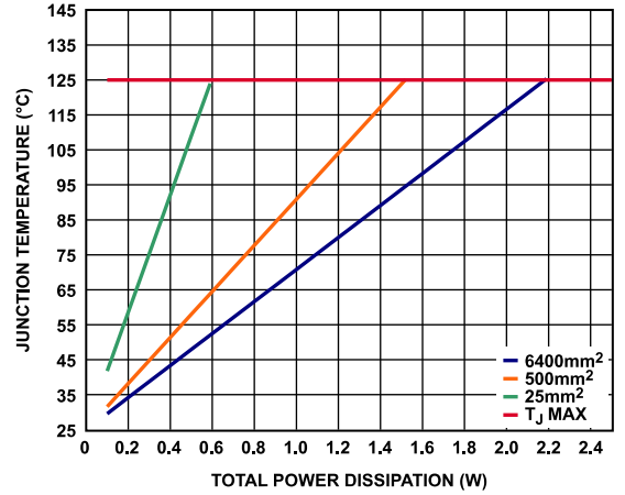
Figure 73. SOIC, T_A = 25^\circ\text{C}
