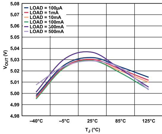
Figure 29. Output Voltage ( V_{OUT} ) vs. Junction Temperature ( T_J ), V_{OUT} = 5\text{ V} , Adjustable
