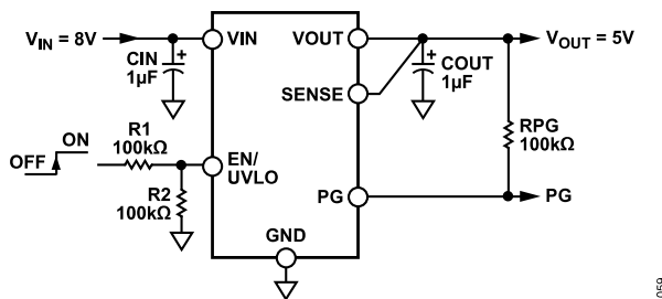
Figure 65. Typical EN Pin Voltage Divider
