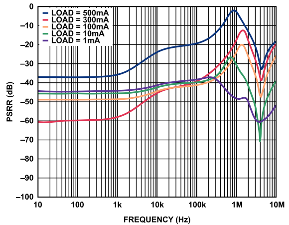
Figure 40. Power Supply Rejection Ratio (PSRR) vs. Frequency, V_{OUT} = 5\text{ V} , V_{IN} = 5.3\text{ V}
