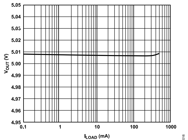
Figure 16. Output Voltage ( V_{OUT} ) vs. Load Current ( I_{LOAD} ), V_{OUT} = 5 V
