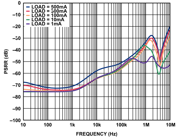
Figure 38. Power Supply Rejection Ratio (PSRR) vs. Frequency, V_{OUT} = 5\text{ V} , V_{IN} = 6\text{ V}
