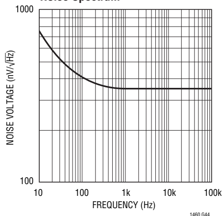
LT1460S3-2.5V Output Voltage Noise Spectrum
