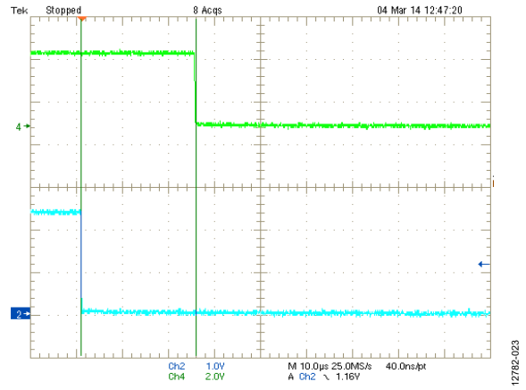
Figure 23. \overline{RESET} Timeout Delay With V_{CC} and V_{IN} Falling
