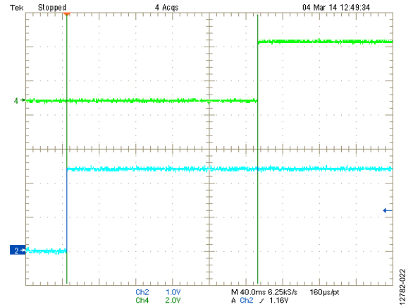
Figure 22. \overline{RESET} Timeout Delay With V_{CC} and V_{IN} Rising
