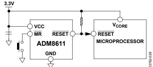
Figure 30. ADM8611 Typical Application Circuit
