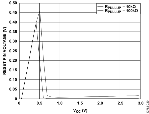
Figure 20. \overline{RESET} Pin Voltage vs. Voltage on VCC (with the \overline{RESET} Pin Pulled Up to the VCC Pin Through R_{PULLUP} )
