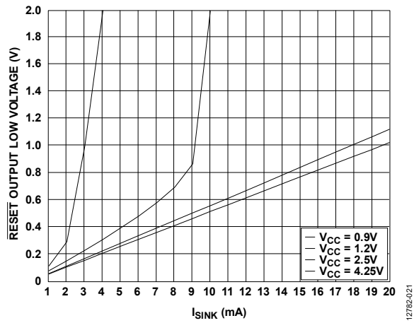
Figure 21. \overline{RESET} Output Low Voltage ( V_{RST\_OL} ) vs. Sink Current ( I_{SINK} )
