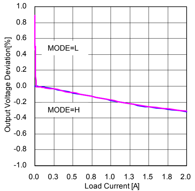
Figure 37. Load Regulation (VIN=5V, VOUT=1.2V, L=1.5μH, FREQ=H)
