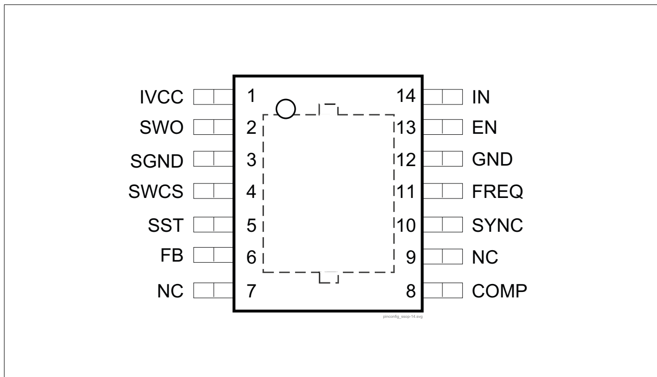
Figure 2 Pin assignment
