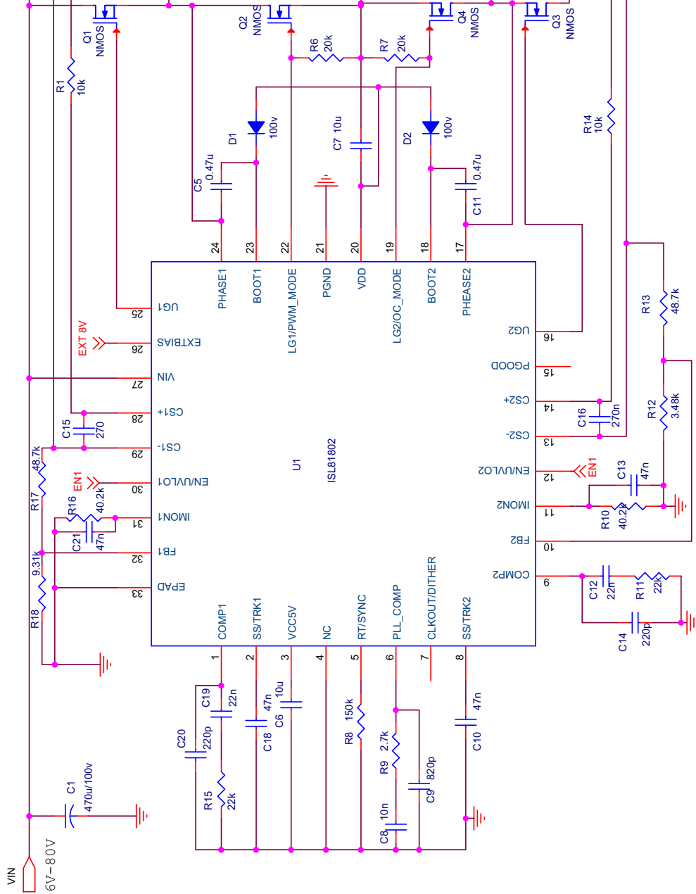
Figure 4. V_{IN} = 18V to 80V , V_{OUT1} = 12V , I_{OUT1} = 10A , V_{OUT2} = 5V , I_{OUT2} = 10A Evaluation Board
