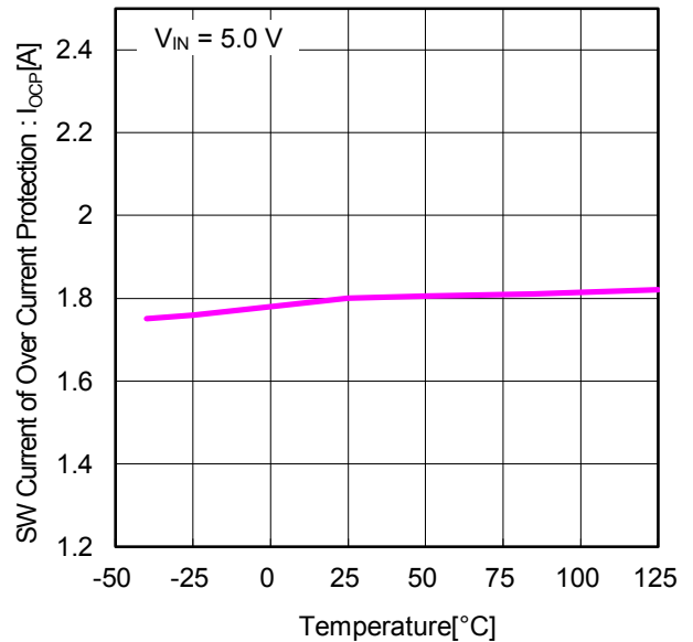
Figure 18 SW Current of Over Current Protection vs Temperature
