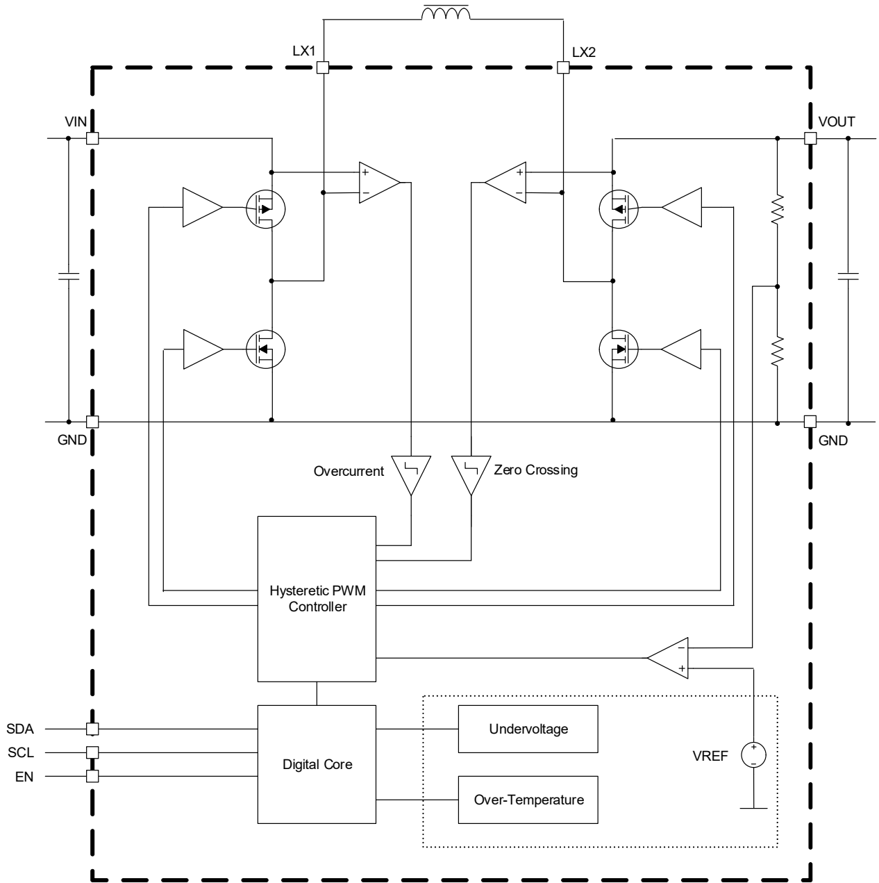
Figure 3. Block Diagram
