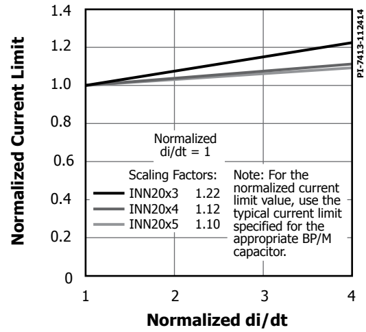
Figure 24. Standard Current Limit Vs. di/dt.
