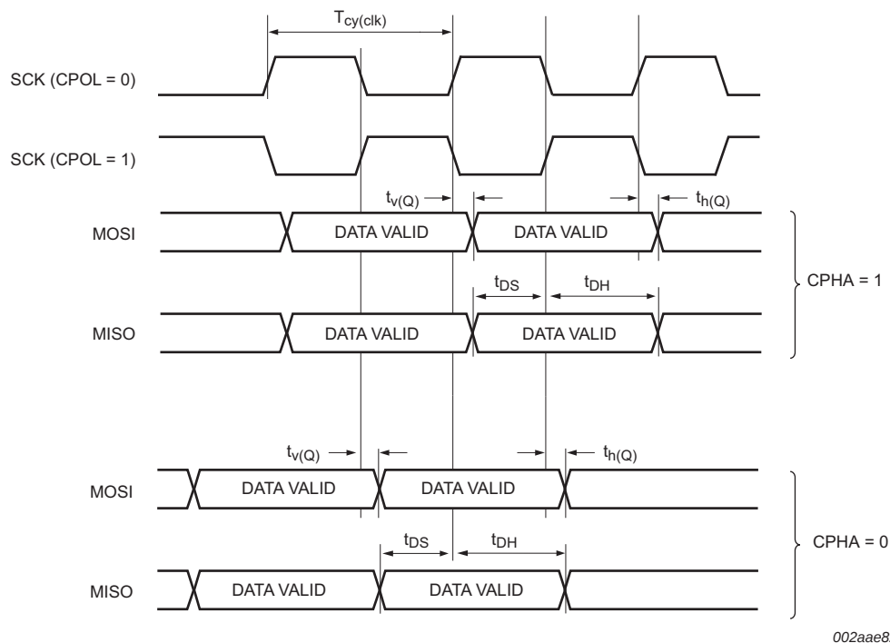
Fig 47. SPI master timing in SPI mode
