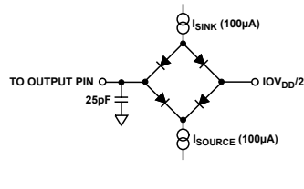
Figure 2. Load Circuit for Timing Characterization
