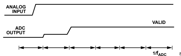
Figure 99. Step Change on the Analog Input, Sinc 4 + Sinc 1 Filter
