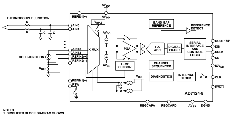
Figure 126. Thermocouple Application
