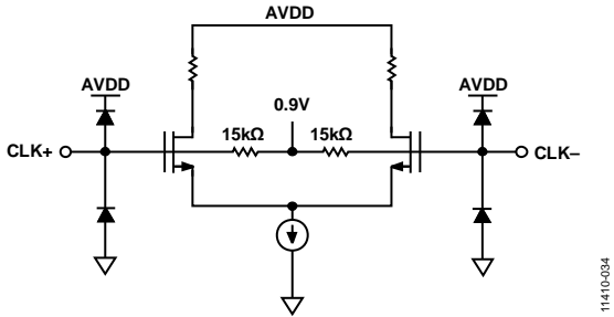
Figure 34. Equivalent Clock Input Circuit
