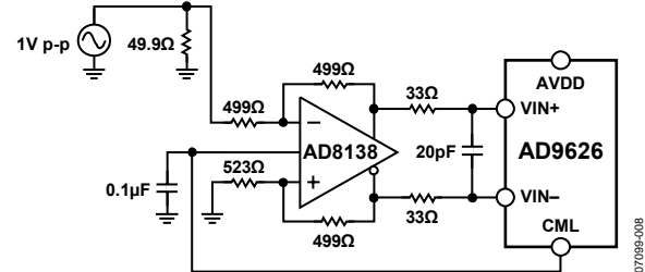
Figure 42. Differential Input Configuration Using the AD8138
