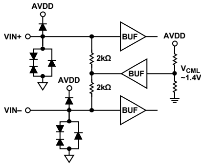
Figure 6. Analog Inputs ( V_{CM} = \sim 1.4V )
