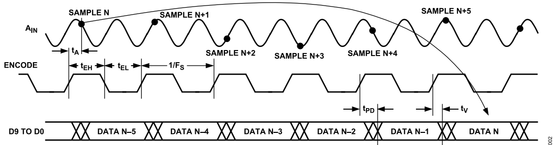
Figure 2. Timing Diagram
