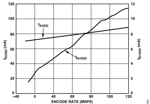
Figure 15. I_{AVDD} and I_{DRVDD} vs. Encode Rate ( f_{AIN} = 10.3 MHz, -0.5 dBFS, and -3 dBFS) C_{LOAD} on Digital Outputs ~7 pF
