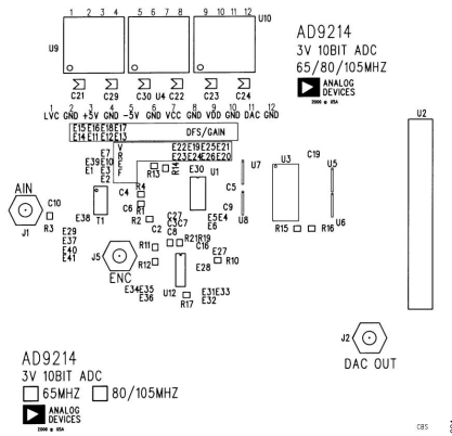
Figure 31. PCB Top Side Silkscreen
