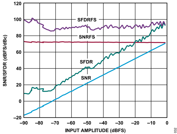
Figure 32. SNR/SFDR vs. Analog Input Level; f_{IN} = 9.7 \text{ MHz} , f_{SAMPLE} = 125 \text{ MSPS}
