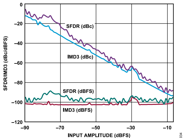
Figure 34. Two-Tone SFDR/IMD3 vs. Input Amplitude (AIN) with f_{IN1} = 70.5 \text{ MHz} and f_{IN2} = 72.5 \text{ MHz} , f_{SAMPLE} = 125 \text{ MSPS}
