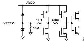
Figure 50. Equivalent VREF Circuit
