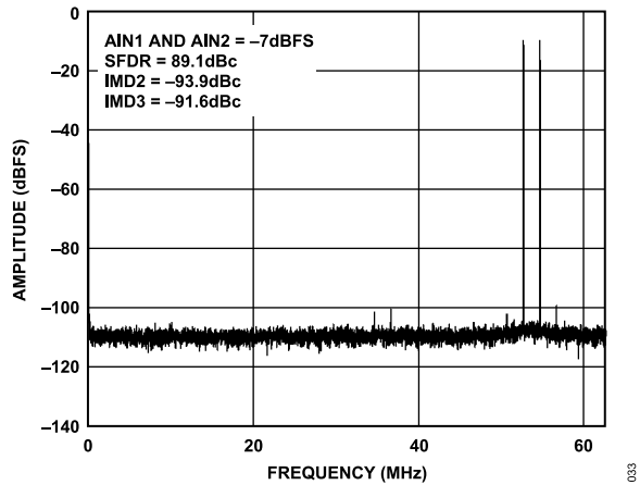
Figure 33. Two-Tone 16k FFT with f_{IN1} = 70.5 \text{ MHz} and f_{IN2} = 72.5 \text{ MHz} , f_{SAMPLE} = 125 \text{ MSPS}
