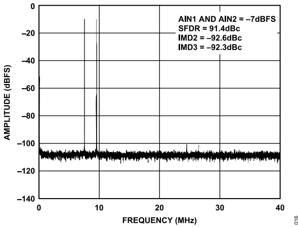
Figure 16. Two-Tone 16k FFT with f_{IN1} = 70.5 \text{ MHz} and f_{IN2} = 72.5 \text{ MHz} , f_{SAMPLE} = 80 \text{ MSPS}
