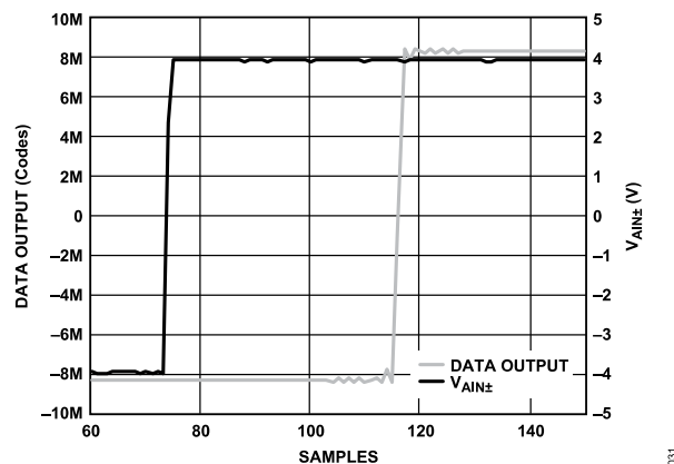
Figure 35. Step Response, Wideband Filter, Wideband 0.433 \times ODR Filter
