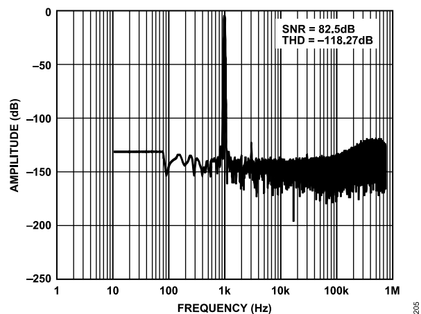
Figure 13. FFT, Low Power Mode, Sinc6 Filter, -0.5 dBFS
