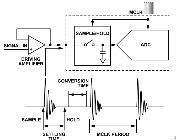
Figure 60. Driving the Input of a Discrete Time ADC
