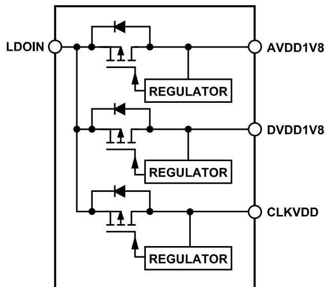
Figure 95. Internal LDO Regulator Connections
