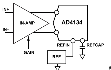
Figure 64. Example Analog Front-End Circuit Design of the AD4134
