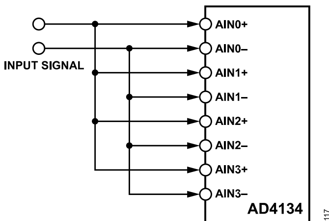
Figure 92. 4:1 Channel Averaging
