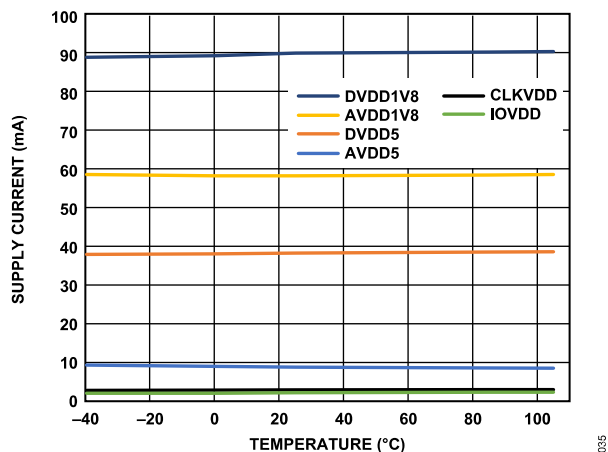
Figure 17. Supply Current vs. Temperature, Wideband 0.433 x ODR Filter
