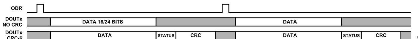
Figure 115. Data CRC Options
