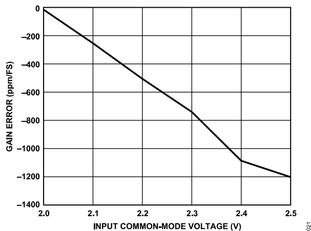
Figure 48. Gain Error vs. Input Common-Mode Voltage, Wideband 0.433 × ODR Filter, High Performance Mode
