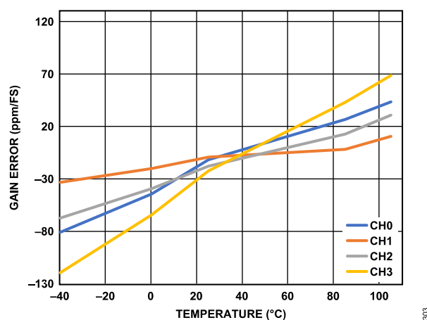
Figure 52. Gain Error vs. Temperature, Wideband 0.433 × ODR Filter, Low Power Mode
