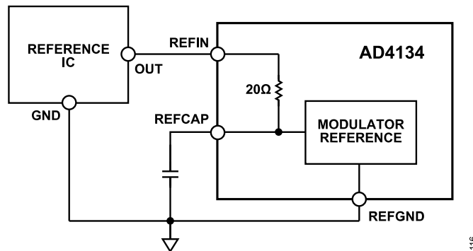
Figure 99. Reference Input Connection Using REFIN Pin
