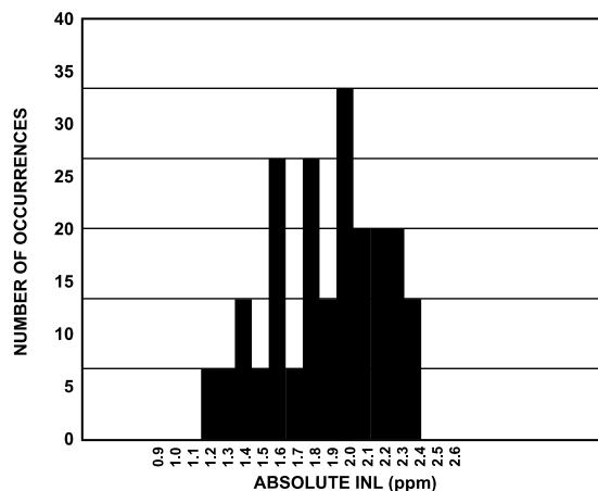
Figure 41. INL Distribution, Wideband 0.433 x ODR Filter, High Performance Mode
