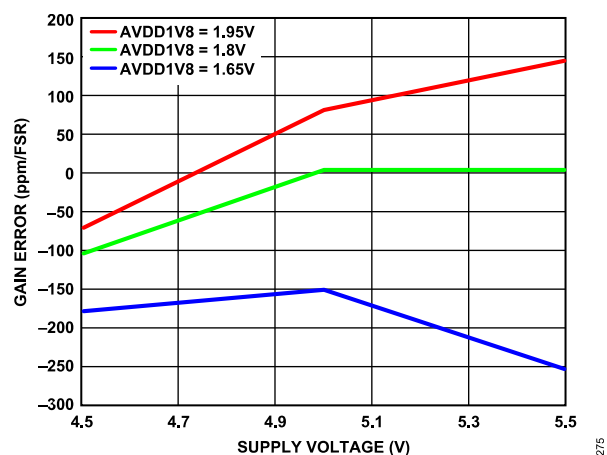
Figure 50. Gain Error vs. Supply Voltage, Wideband 0.433 × ODR Filter, High Performance Mode
