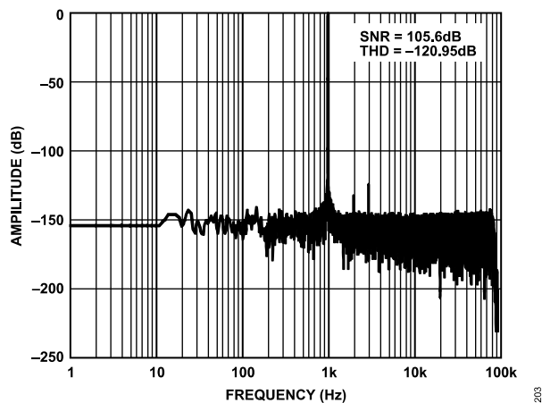
Figure 12. FFT, Low Power Mode, Wideband 0.433 x ODR Filter, -0.5 dBFS, ODR = 187 kSPS
