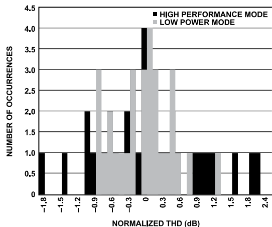
Figure 21. THD Histogram
