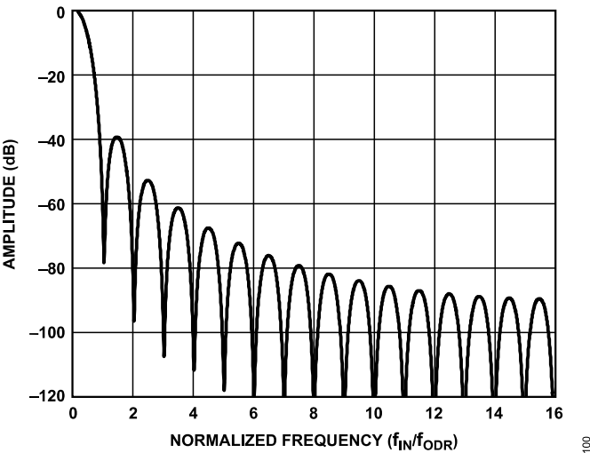
Figure 77. Sinc3 Filter Frequency Response
