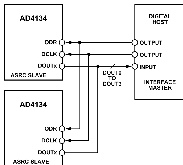
Figure 117. Data interface Example 2, Two AD4134 Devices in ASRC Slave Mode with Digital Host as Interface Master
