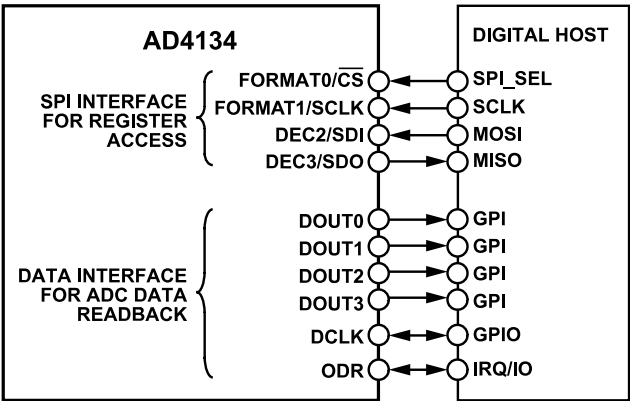
Figure 108. Communication Interface of AD4134
