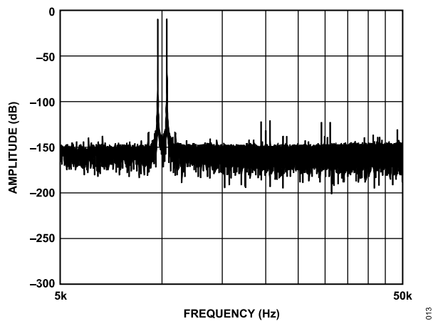
Figure 15. IMD with Input Signals at 9.7 kHz and 10.3 kHz, Wideband 0.433 x ODR Filter
