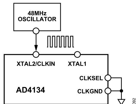
Figure 69. Master Clock Provided by an Oscillator
