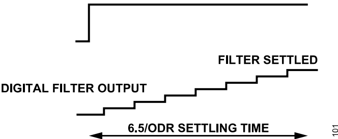
Figure 78. Sinc6 Filter Step Response
