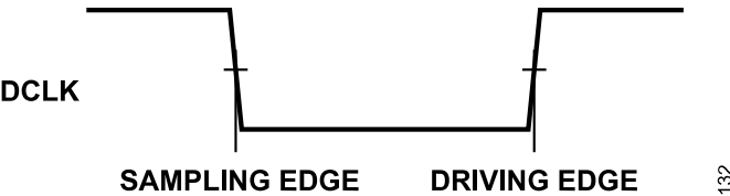
Figure 114. DCLK Edges
