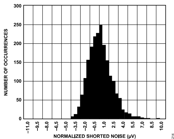
Figure 28. Shorted Noise, Sinc3 Filter, High Performance Mode
