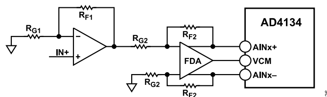
Figure 107. Op Amp and Fully Differential Amplifier
