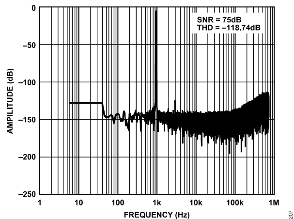
Figure 14. FFT, Low Power Mode, Sinc3 Filter, -0.5 dBFS
