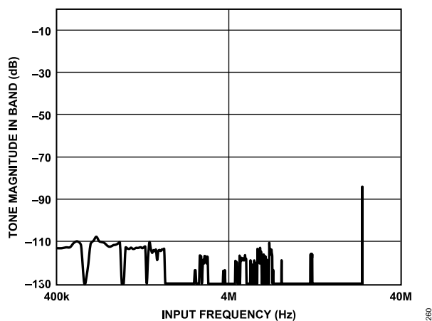
Figure 32. Tone Magnitude In Band vs. Input Frequency, 4 V p-p Input Signal, Wideband 0.433 \times ODR Filter, High Performance Mode
