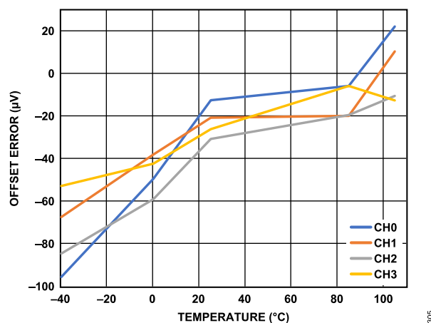
Figure 45. Offset Error vs. Temperature, Wideband 0.433 × ODR Filter, Low Power Mode
