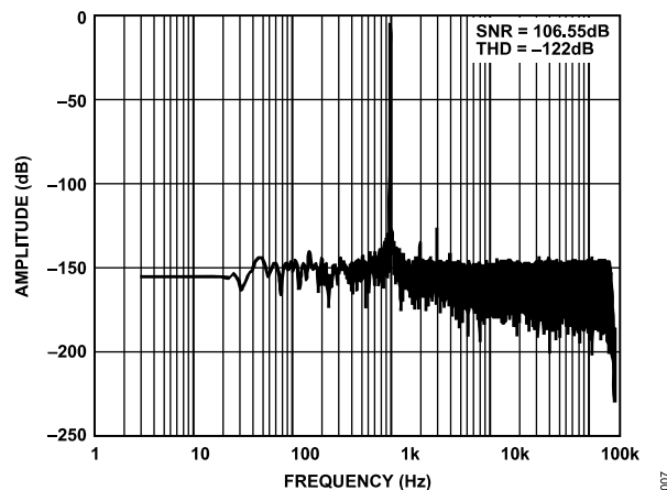
Figure 9. FFT, High Performance Mode, -0.5\text{ dBFS} , Wideband 0.433 \times \text{ODR} Filter, \text{ODR} = 374\text{ kSPS}
