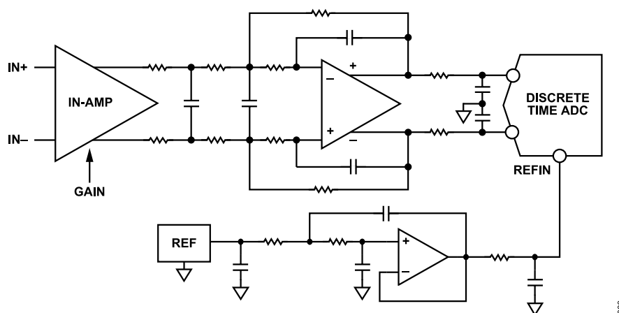
Figure 63. Example Analog Front-End Circuit Design of the Discrete Time-Based ADC
