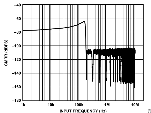
Figure 53. CMRR vs. Input Frequency, Wideband 0.433 × ODR Filter, High Performance Mode
