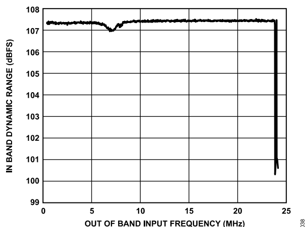
Figure 31. In Band Dynamic Range vs. Out of Band Input Frequency of 1 V p-p Input Signal, Wideband 0.433 \times ODR Filter, High Performance Mode
