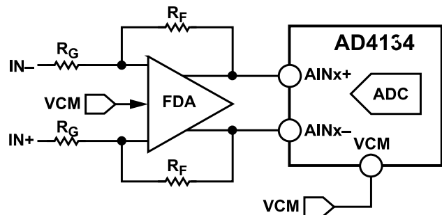
Figure 103. Use a Fully Differential Amplifier to Extend Input Common-Mode Voltage and Signal Gain/Attenuation
