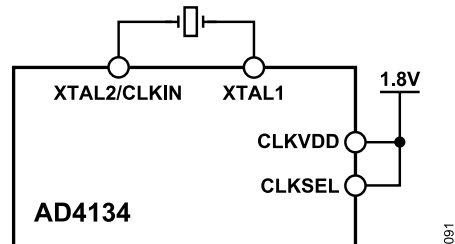
Figure 68. Master Clock Provided by a Crystal
