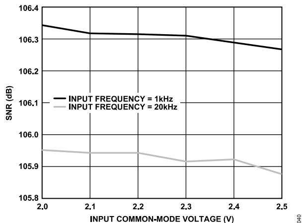
Figure 23. SNR vs. Input Common-Mode Voltage, Wideband 0.433 × ODR Filter
