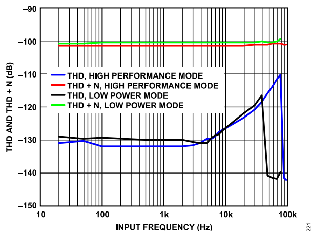
Figure 19. THD and THD + N vs. Input Frequency, -6 dBFS Input, 0.433 × ODR Filter
