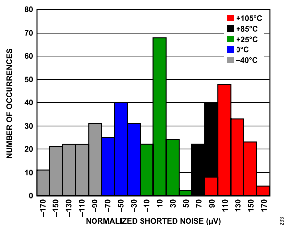
Figure 49. Gain Error Distribution, Wideband 0.433 × ODR Filter, High Performance Mode
