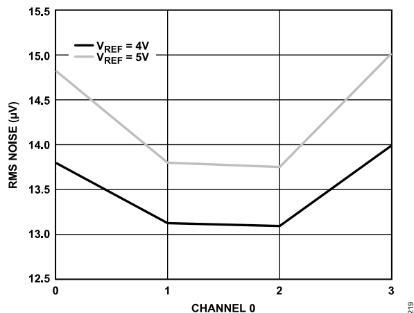
Figure 30. RMS Noise per Channel for Various V_{REF} Values, Wideband 0.433 \times ODR Filter, Low Power Mode
