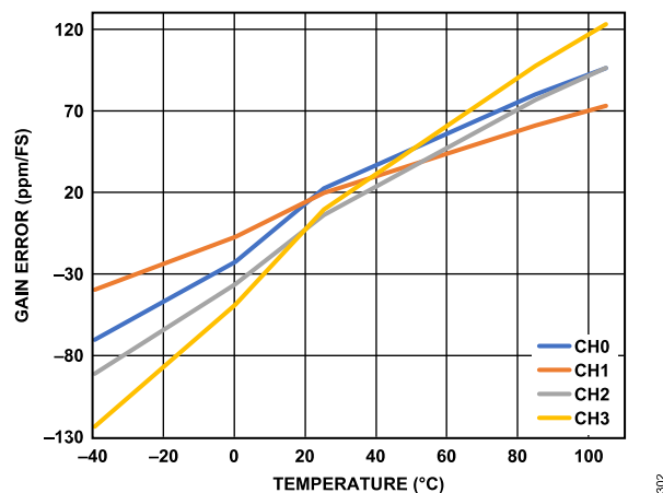
Figure 51. Gain Error vs. Temperature, Wideband 0.433 × ODR Filter, High Performance Mode
