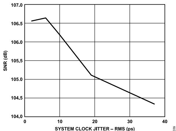
Figure 22. SNR vs. System Clock Jitter, Wideband 0.433 × ODR Filter
