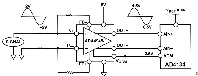
Figure 104. Fully Differential Amplifier with Single Supply
