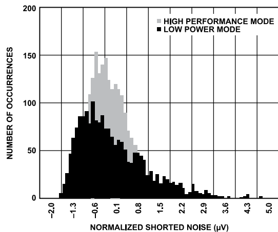
Figure 27. Shorted Noise, 0.433 × ODR Filter
