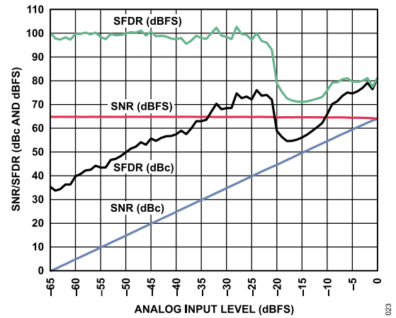
Figure 23. SNR/SFDR vs. Analog Input Level, f_{IN} = 170.3\text{ MHz} , Buffer Current = 3.5\times
