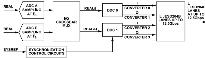
Figure 79. Two-ADC Plus Two-DDC Mode
