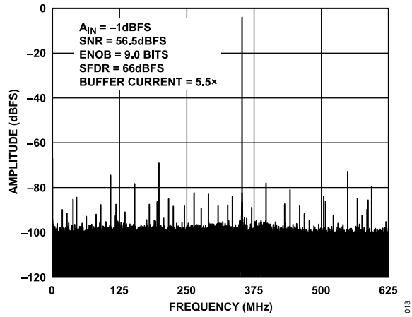
Figure 13. Single-Tone FFT with f_{IN} = 1600.3 MHz
