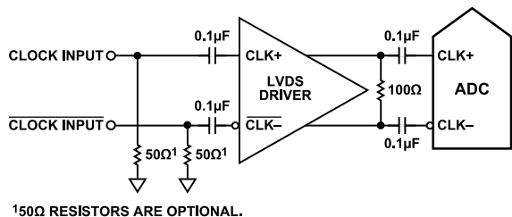
Figure 52. Differential LVDS Sample Clock
