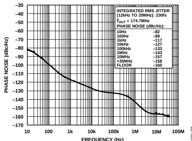
Figure 8. Absolute Phase Noise (PLL0, Configuration 6, HCSSL Mode, f_{REF} = 155.52\text{MHz} , f_{OUT} = 174.7\text{MHz} , f_{SYS} = 52\text{MHz} Crystal, BW_{DPLL} = 50\text{Hz} , Phase Buildout Mode)
