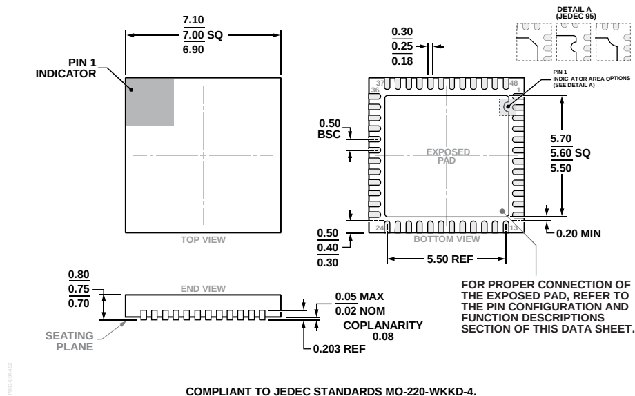
Figure 65. 48-Lead Lead Frame Chip Scale Package [LFCSP] 7 mm × 7 mm Body and 0.75 mm Package Height (CP-48-13)
