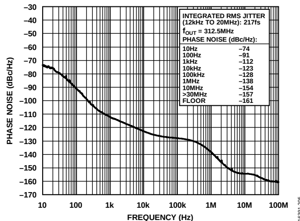
Figure 7. Absolute Phase Noise (PLL0, Configuration 5, HCSSL Mode, f_{REF} = 25\text{MHz} , f_{OUT} = 312.5\text{MHz} , f_{SYS} = 52\text{MHz} Crystal, BW_{DPLL} = 50\text{Hz} , Phase Buildout Mode)
