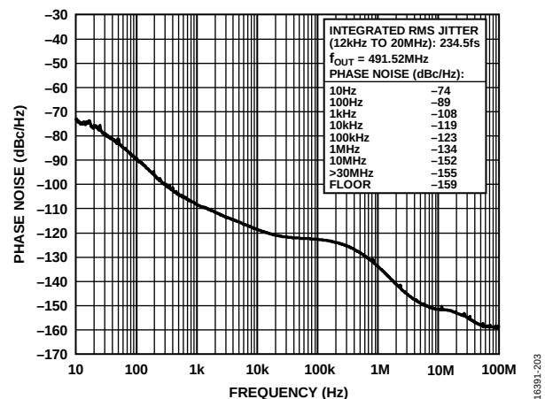
Figure 5. Absolute Phase Noise (PLL0, Configuration 3, HCSSL Mode, f_{REF} = 1\text{Hz} , f_{OUT} = 491.52\text{MHz} , f_{COMP} = 19.2\text{MHz} TCXO, f_{SYS} = 52\text{MHz} Crystal, BW_{DPLL} = 50\text{Hz} )
