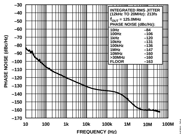
Figure 6. Absolute Phase Noise (PLL0, Configuration 4, HCSSL Mode, f_{REF} = 125\text{MHz} , f_{OUT} = 125.0\text{MHz} , f_{COMP} = 19.2\text{MHz} TCXO, f_{SYS} = 52\text{MHz} Crystal, BW_{DPLL} = 0.1\text{Hz} , Phase Buildout Mode)
