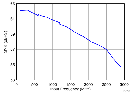
Figure 36. Signal-to-Noise Ratio vs Input Frequency
