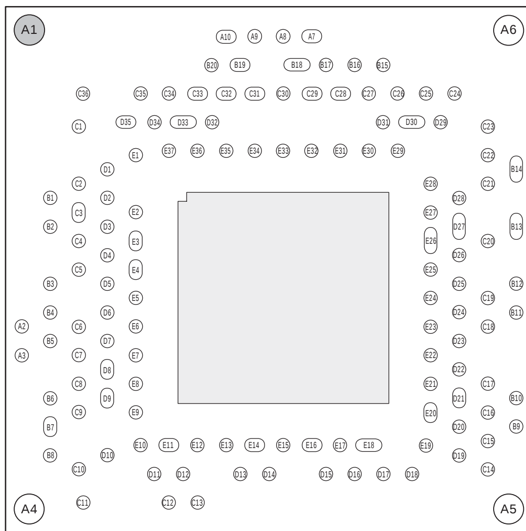
Figure 22 • Pin Diagram
