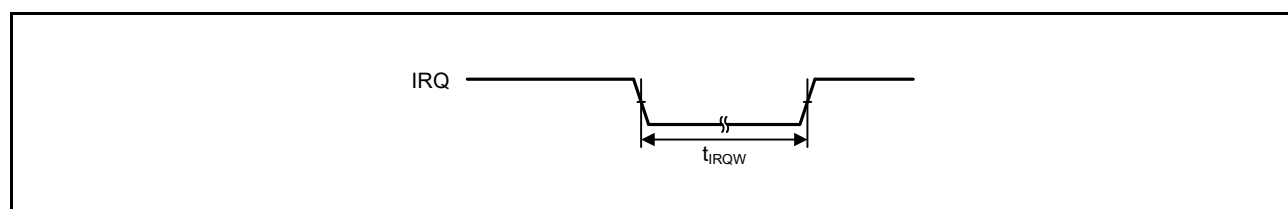
Figure 47.35 IRQ interrupt input timing
