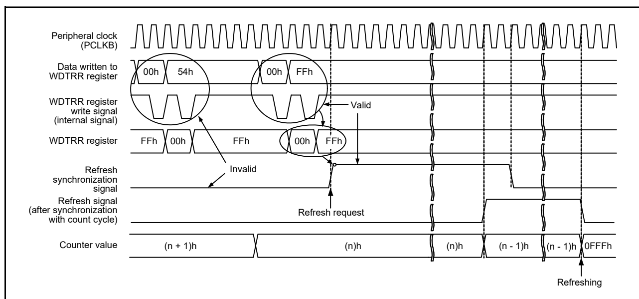
Figure 24.6 WDT refresh operation waveforms when \text{WDTCR.CKS}[3:0] = 0100b , \text{WDTCR.TOPS}[1:0] = 01b
