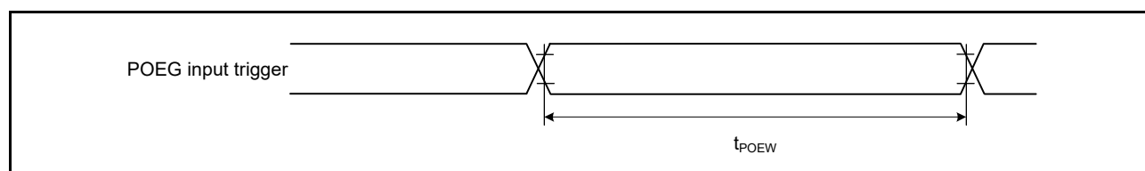
Figure 47.37 POEG input trigger timing
