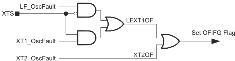
Figure 5-8. Oscillator-Fault Logic
