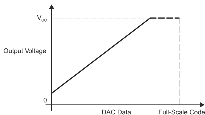
Figure 25-5. Positive Offset
