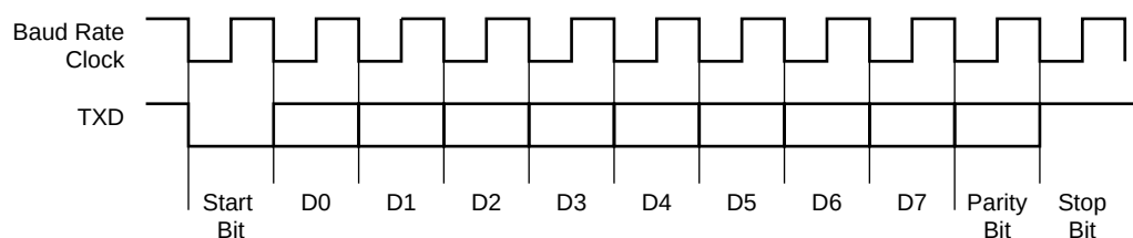
Figure 20-3. Character Transmit
