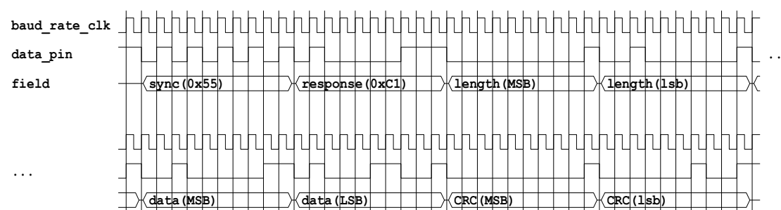
Figure 31-7. Example Response
