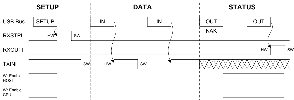
Figure 19-7. Control Read
