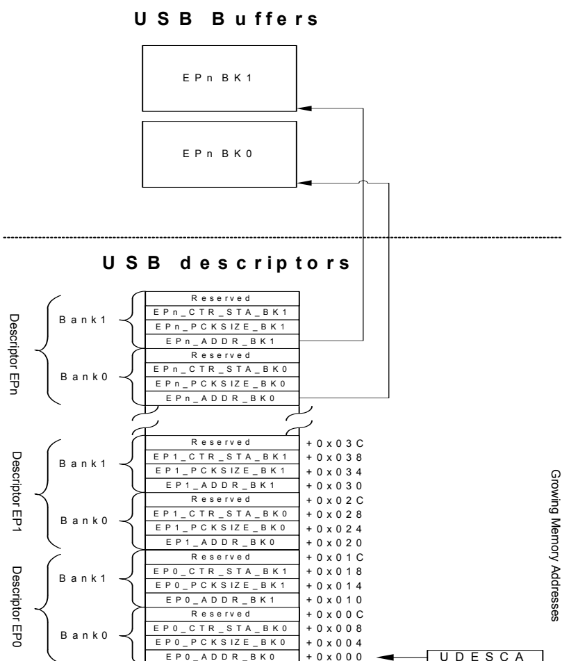
Figure 19-5. Memory organization
