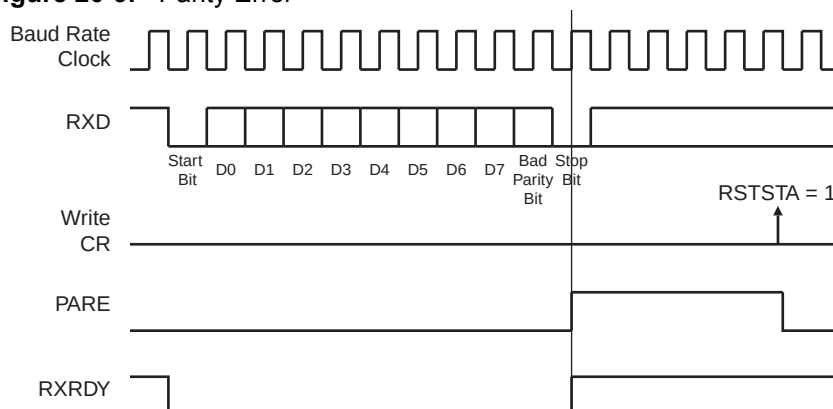
Figure 20-9. Parity Error
