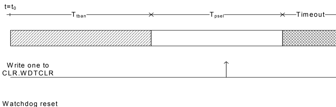
Figure 15-4. Window Mode WDT Timing Diagram
