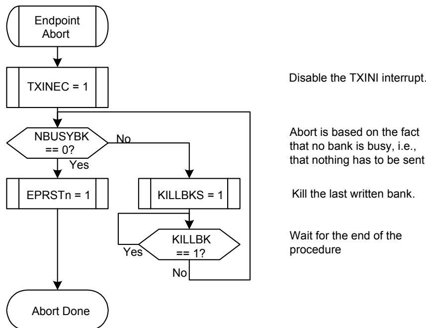
Figure 19-10. Abort Algorithm
