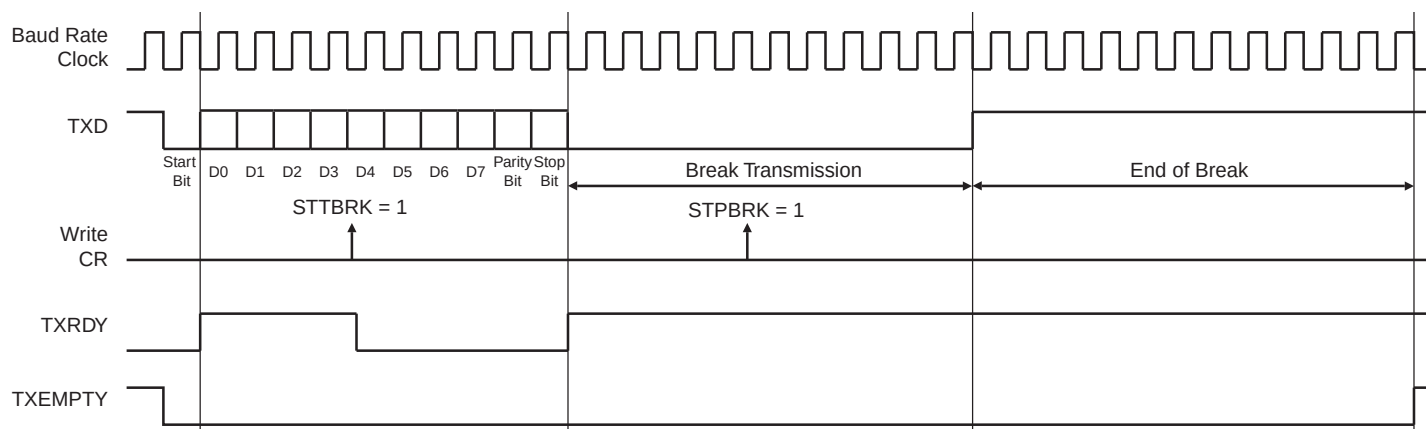
Figure 20-13. Break Transmission
