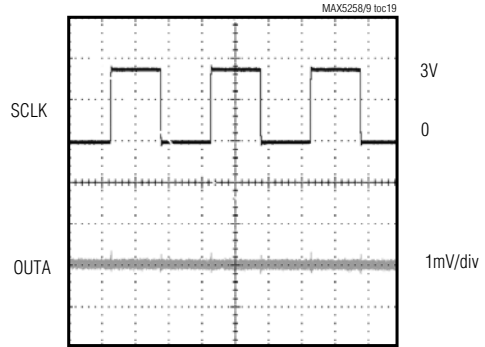
CLOCK FEEDTHROUGH
