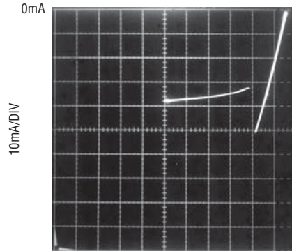
Short-Circuit Output Current vs V_{OUT} (Sourcing)
