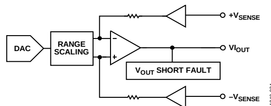
Figure 75. Voltage Output
