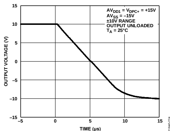
Figure 23. Full-Scale Negative Step
