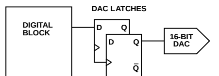
Figure 83. DAC Data Integrity
