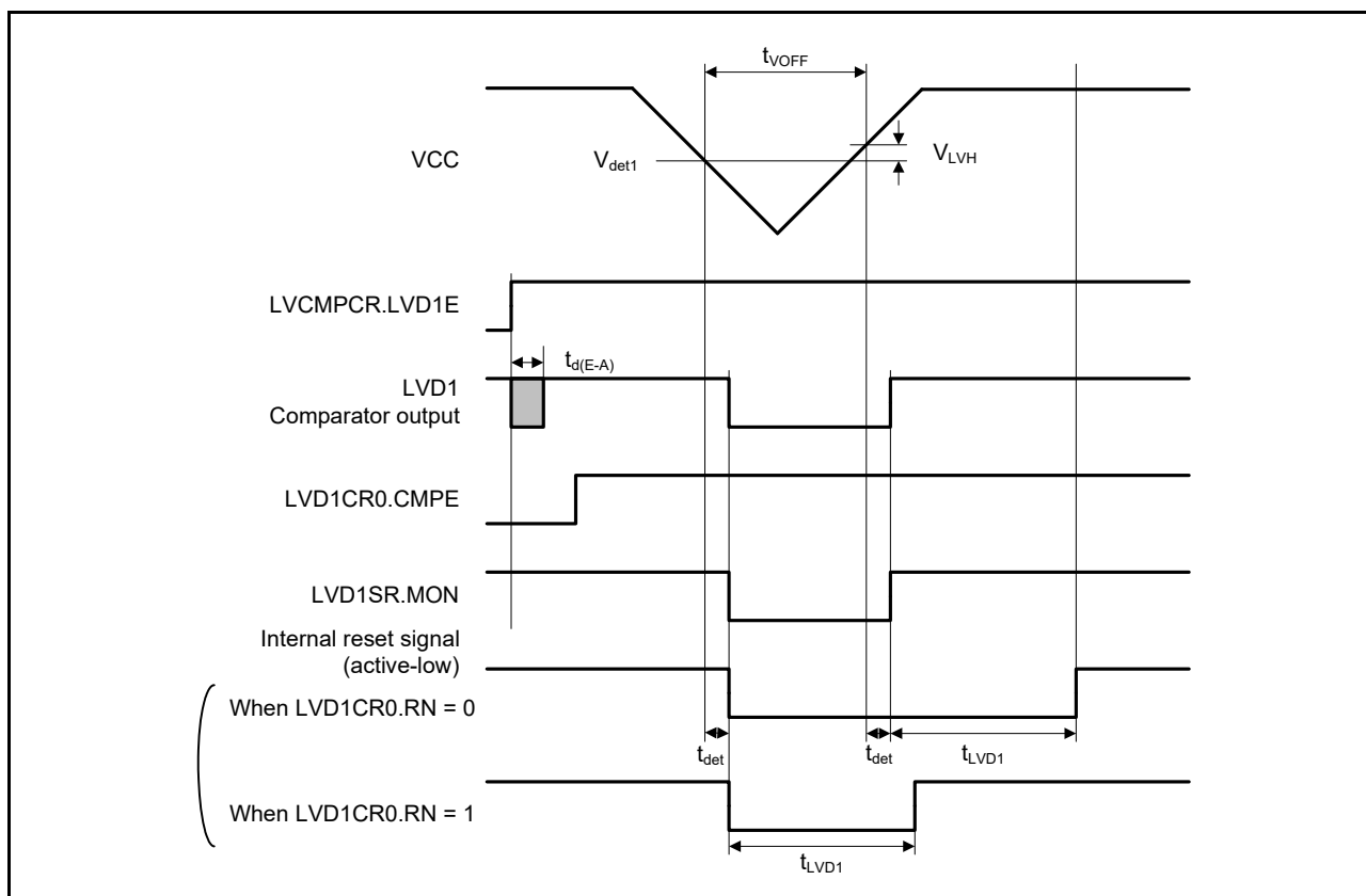
Figure 2.99 Voltage detection circuit timing ( V_{\text{det1}} )
