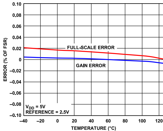
Figure 12. Gain Error and Full-Scale Error vs. Temperature
