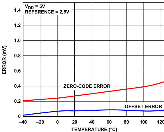
Figure 13. Zero-Code Error and Offset Error vs. Temperature
