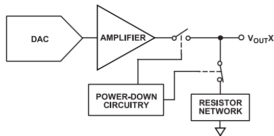
Figure 39. Output Stage During Power-Down
