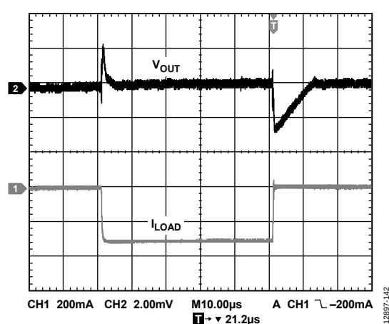
Figure 39. Load Transient Response, V_{OUT} = -2.5\text{ V} , I_{LOAD} = -10\text{ mA to } -300\text{ mA}
