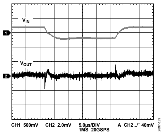
Figure 36. Line Transient Response, 500 mV Step, V_{OUT} = -1.2\text{ V} , I_{LOAD} = -300\text{ mA}
