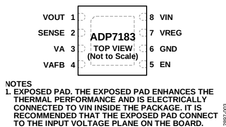
Figure 3. Pin Configuration
