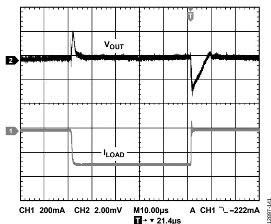
Figure 38. Load Transient Response, V_{OUT} = -1.2\text{ V} , I_{LOAD} = -10\text{ mA to } -300\text{ mA}
