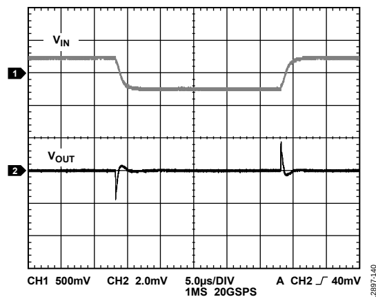
Figure 37. Line Transient Response, 500 mV Step, V_{OUT} = -3.3\text{ V} , I_{LOAD} = -300\text{ mA}
