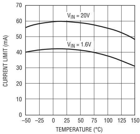
Current Limit
