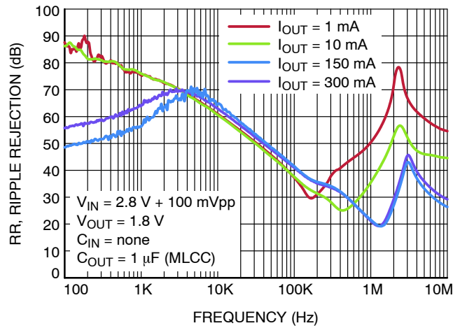
Figure 25. Power Supply Rejection Ratio, V_{OUT} = 1.8\text{ V}
