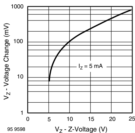
Fig. 3 - Typical Change of Working Voltage under Operating Conditions at T_{\text{amb}} = 25^\circ\text{C}
