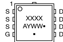
WDFN8 ( \mu 8\text{FL} ) CASE 511AB
